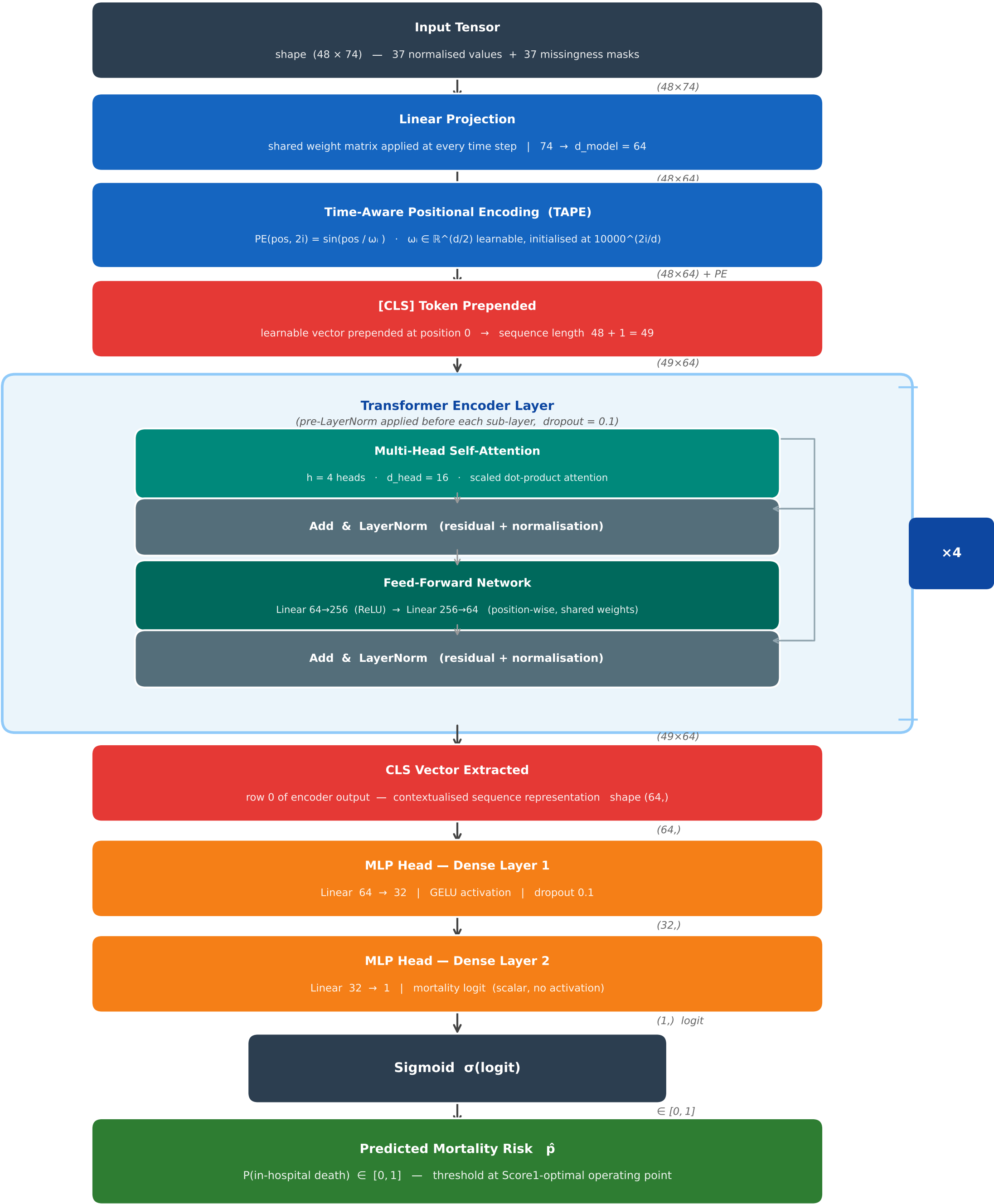
Figure 2.2 — Time-Aware Transformer Architecture
