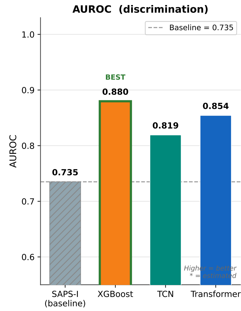
Figure — Final Model Comparison: XGBoost · TCN · Time-Aware Transformer vs SAPS-I Clinical Baseline PhysioNet 2012 Set-A | 600-patient held-out test split | 13.5% mortality
