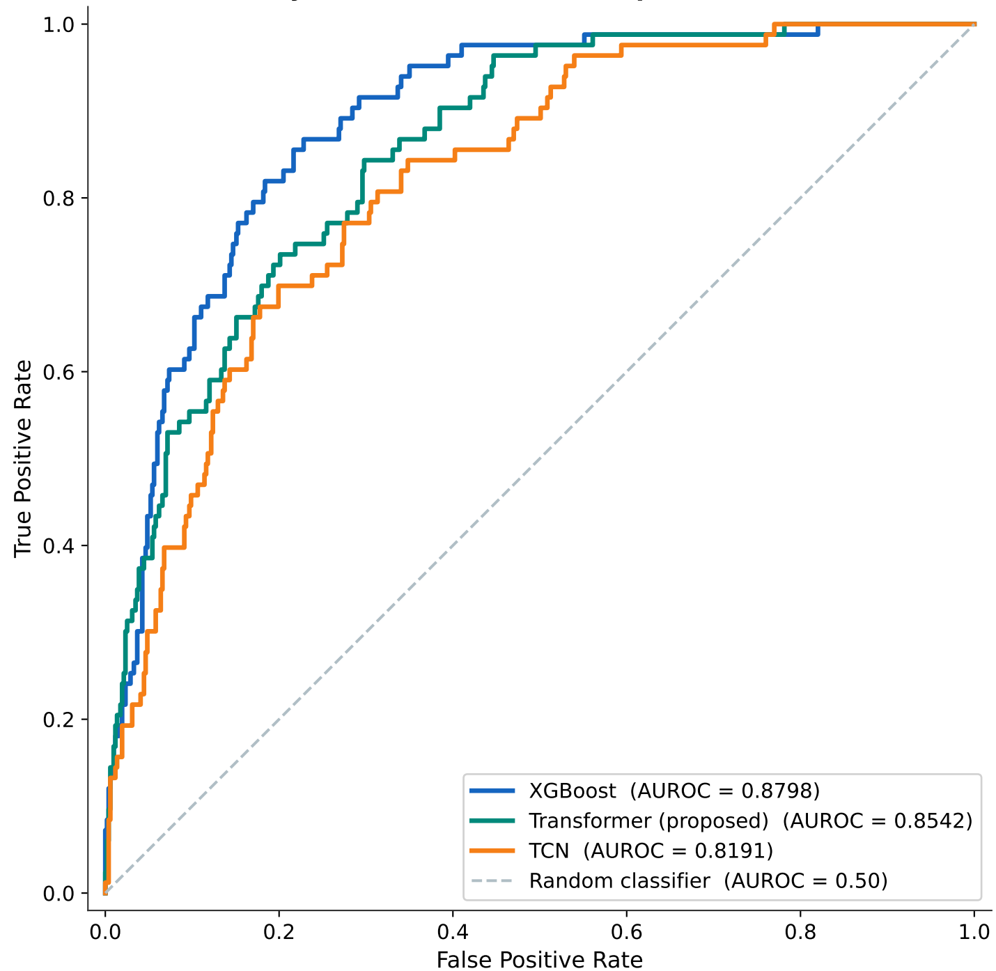
Figure 5.1 — ROC Curves: Model Comparison PhysioNet 2012 Set-A test split (n = 600)
