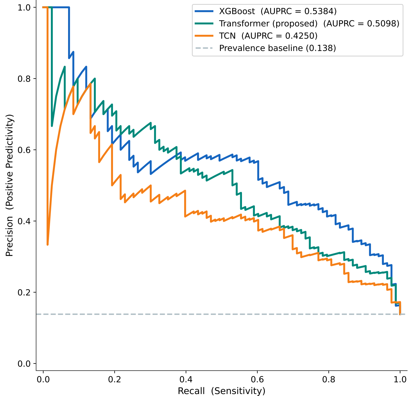
Figure 5.2 — Precision-Recall Curves: Model Comparison PhysioNet 2012 Set-A test split (n = 600)
