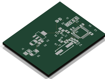
reports/renderers/stm32-blinky_iso.png
