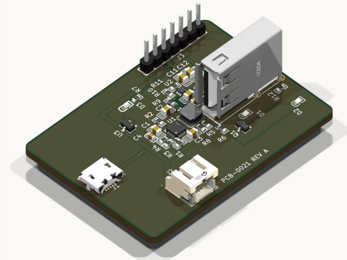
LIPO-BOOST 2 LAYERS · 53.9 × 38.8 MM · 33 FOOTPRINTS VERIFICATION, FINDINGS OPEN
