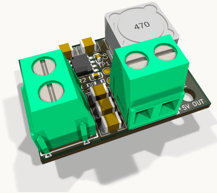
BB-BUCK 2 LAYERS · 35 × 25 MM · 20 FOOTPRINTS PACKAGE READY
