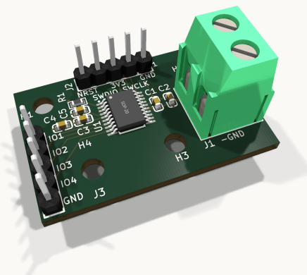
BB-MCU 2 LAYERS · 34.8 × 22.3 MM · 14 FOOTPRINTS PACKAGE READY
