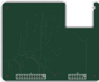
reports/renders/lumina-par_bottom.png
