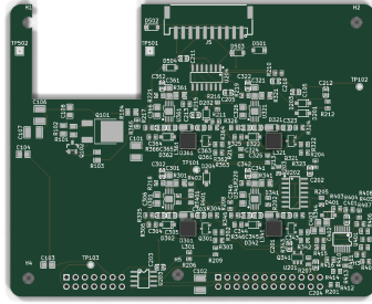
reports/renders/lumina-par_top.png
