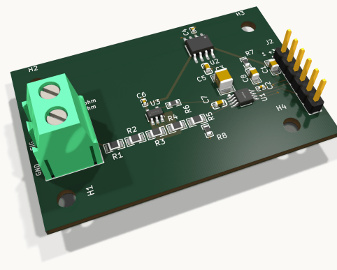
BB-ADC 2 LAYERS · 54.8 × 34.9 MM · 25 FOOTPRINTS
