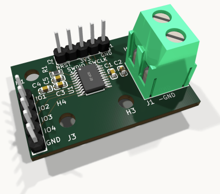
BB-MCU 2 LAYERS · 34.8 × 22.3 MM · 14 FOOTPRINTS
