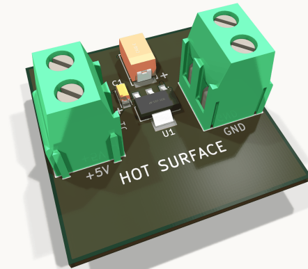
BB-LDO 2 LAYERS · 34.7 × 34.7 MM · 5 FOOTPRINTS
