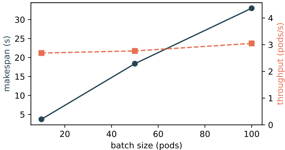
Scheduler scalability (kind, N=10/batch)
