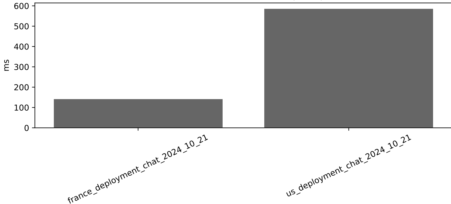
E6 Live Azure Validation Latency Snapshot
