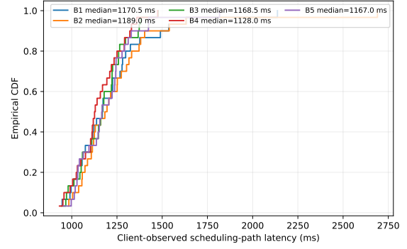
Fig. 1. AKS B1–B5 scheduling-latency CDF using one comparable instrument: high-resolution client-observed scheduling-path timing. B5’s separate scheduler-internal phase timing is reported only in text, not mixed into this CDF. Warmups are retained in raw data but excluded from this figure.
