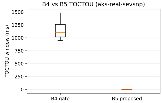
Fig. 2. Central result: the strong scheduling-gate baseline B4 leaves a \sim 1.1 s externally controllable gate-removal-to-bind window; our fail-closed PreBind design removes that window from the schedulable path ( N=30 ; p < 10^{-5} , Cliff’s \delta=1.0 ).
