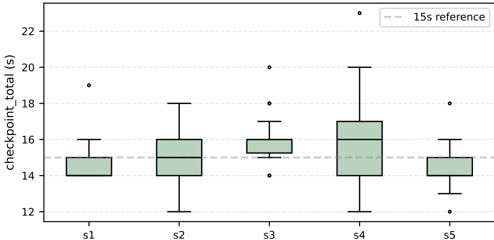
RQ3 — checkpoint cost envelope across 5 stacks
