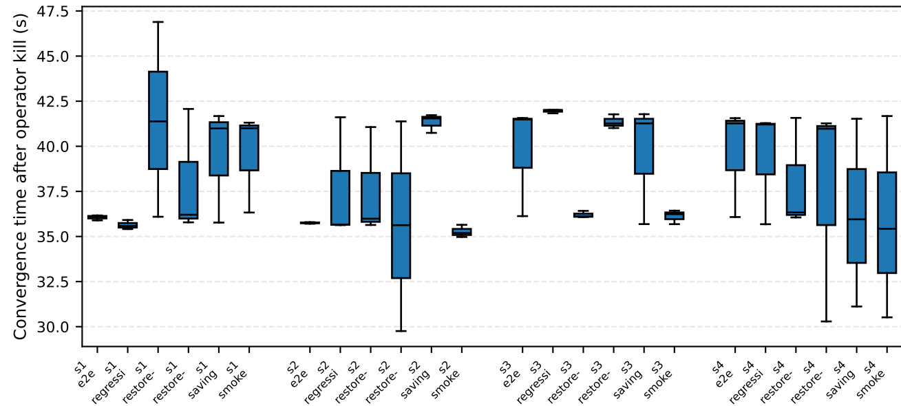
RQ5 — convergence time per subject x kill_step
