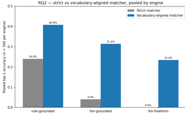
Figure 5: Pooled top-1 by engine on S1 ( n = 500 per engine). Gray bars show strict matching; blue bars show vocabulary-aligned matching.
