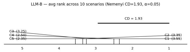
Figure 9: Critical-difference diagram for LLM-B (cohere-command-a). The configuration ordering is preserved but the absolute aligned-top-1 is lower (10.4 % pooled vs 22.4 % for LLM-A).
