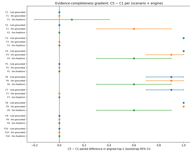
Figure 7: Per-scenario C5 - C1 aligned top-1 gain. Positive points indicate that fuller evidence helps; intervals show bootstrap 95 % CIs.
