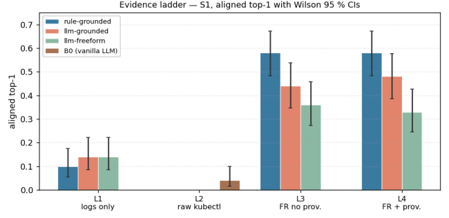
Figure 4: Evidence ladder L1 \rightarrow L4 on S1, aligned top-1 with Wilson 95 % CIs. L1 (logs only) and L2 (raw kubect1) are at the floor; the large jump is to L3 (FailureReport typed bundle); L4 (+ PROV graph) adds little on top of L3.
