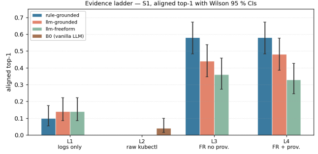
Figure 3: Aligned top-1 on the L1–L4 evidence ladder (S1, Wilson 95 % CI). Larger gain crossing L2→L3 than crossing L3→L4: operator-side typing dominates; the PROV graph contributes marginally.
