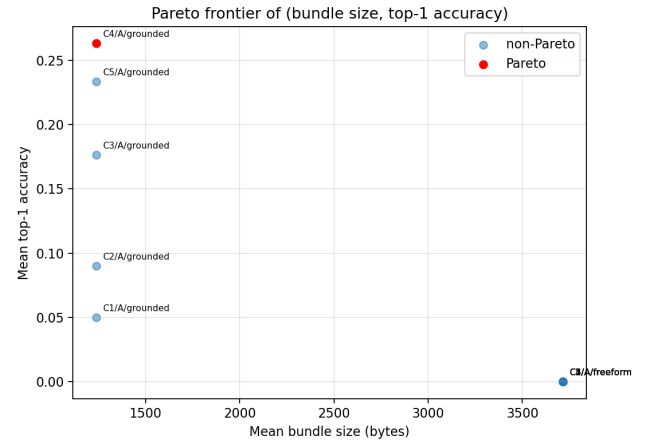
Figure 10: Pareto frontier: bundle size (B, x-axis) vs aligned top-1 (y-axis). The red point is the cell that no other strictly dominates.
