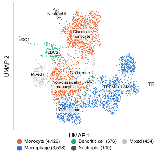
A Myeloid sub-clusters (Harmony)
