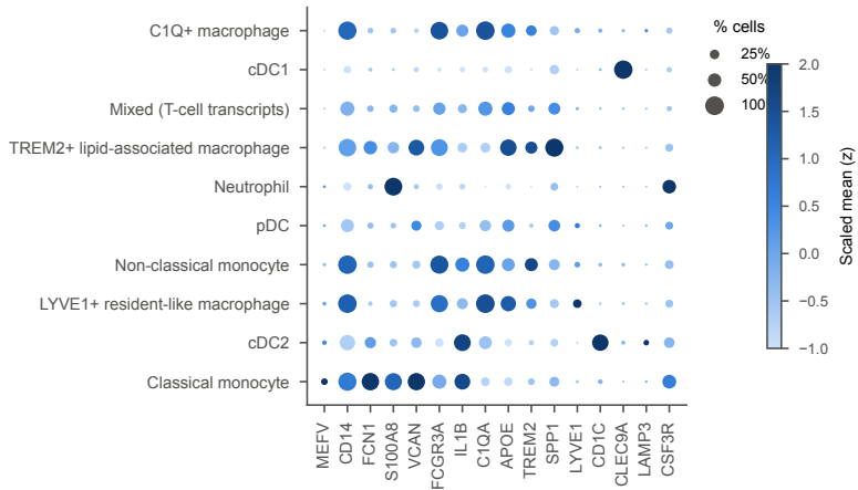
Marker detection (size) and scaled mean (colour)
