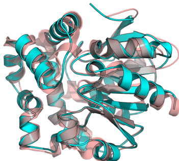
A FAcD Fold Superposition (MSLW1 vs. 8SDC) B Active-Site Catalytic Triad Alignment TM-score = 0.985, RMSD = 0.99 Å (cyan / salmon) Asp104 - His271 - Asp128 (sticks; N blue, O red)
