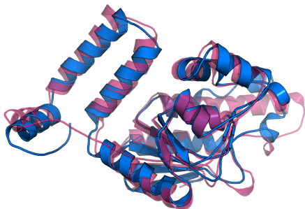
C Chlorobenzoyl-CoA Dehalogenase (PHW2 vs. DNEKD) D Dehalogenase Fold (PHW1 vs. 3UMG) TM-score = 0.939, RMSD = 2.04 Å (marine / pink) TM-score = 0.946, RMSD = 1.71 Å (green / wheat)
