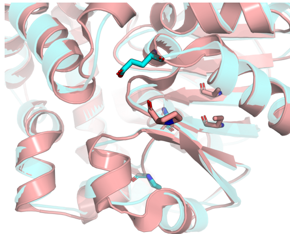
A FAcD Fold Superposition (MSLW1 vs. 8SDC) B Active-Site Catalytic Triad Alignment TM-score = 0.985, RMSD = 0.99 Å (cyan / salmon) Asp104 - His271 - Asp128 (sticks; N blue, O red)
