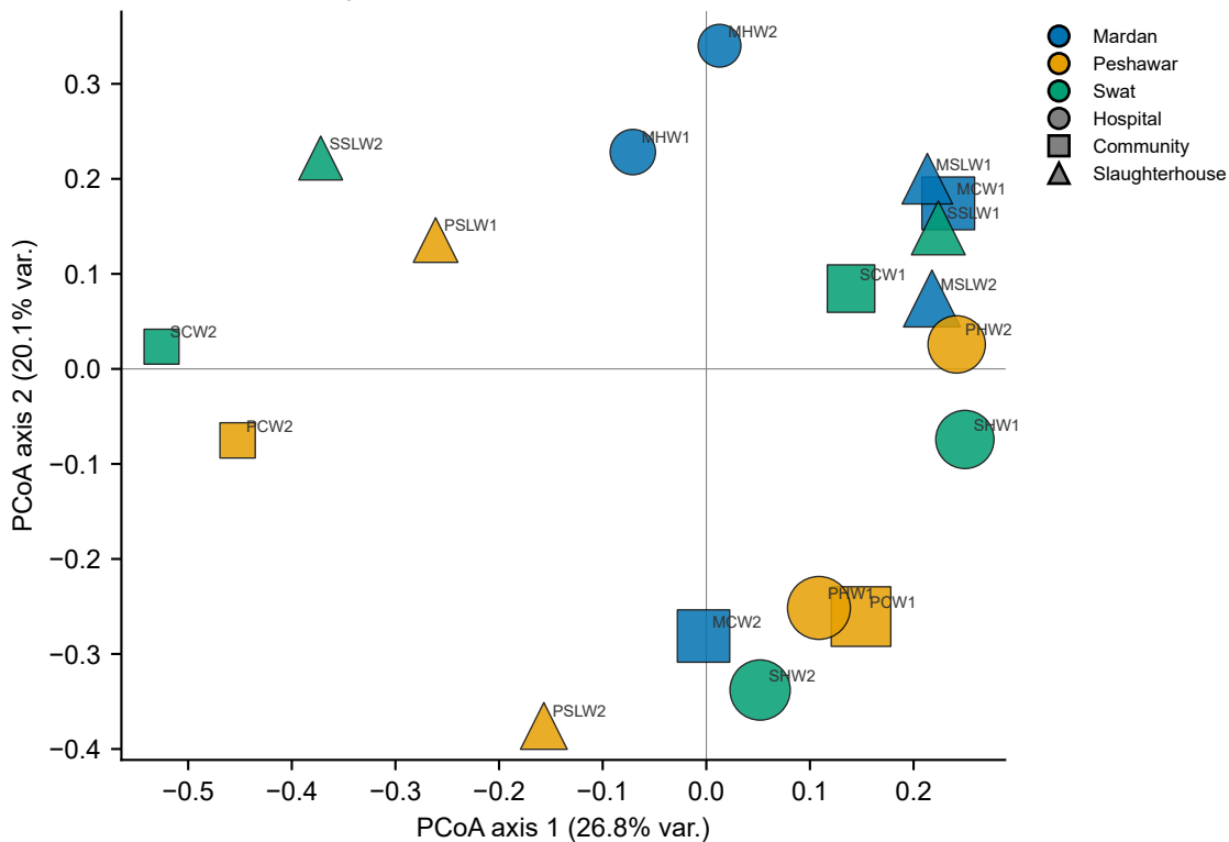
Community structure (Bray-Curtis PCoA) with candidate-gene abundance overlay (marker size)
