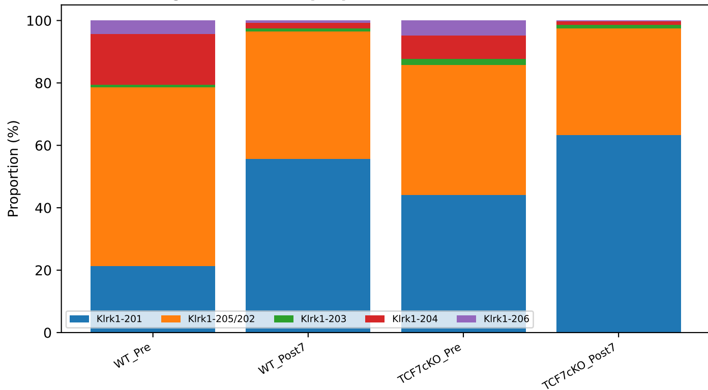
FigV3 — Isoform proportions (GSE203167, 5 units)
