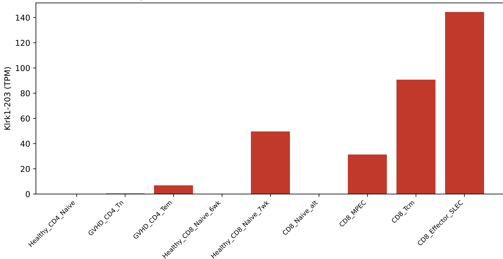
Fig1 — Klrk1-203 (ENSMUST00000137660) induction
