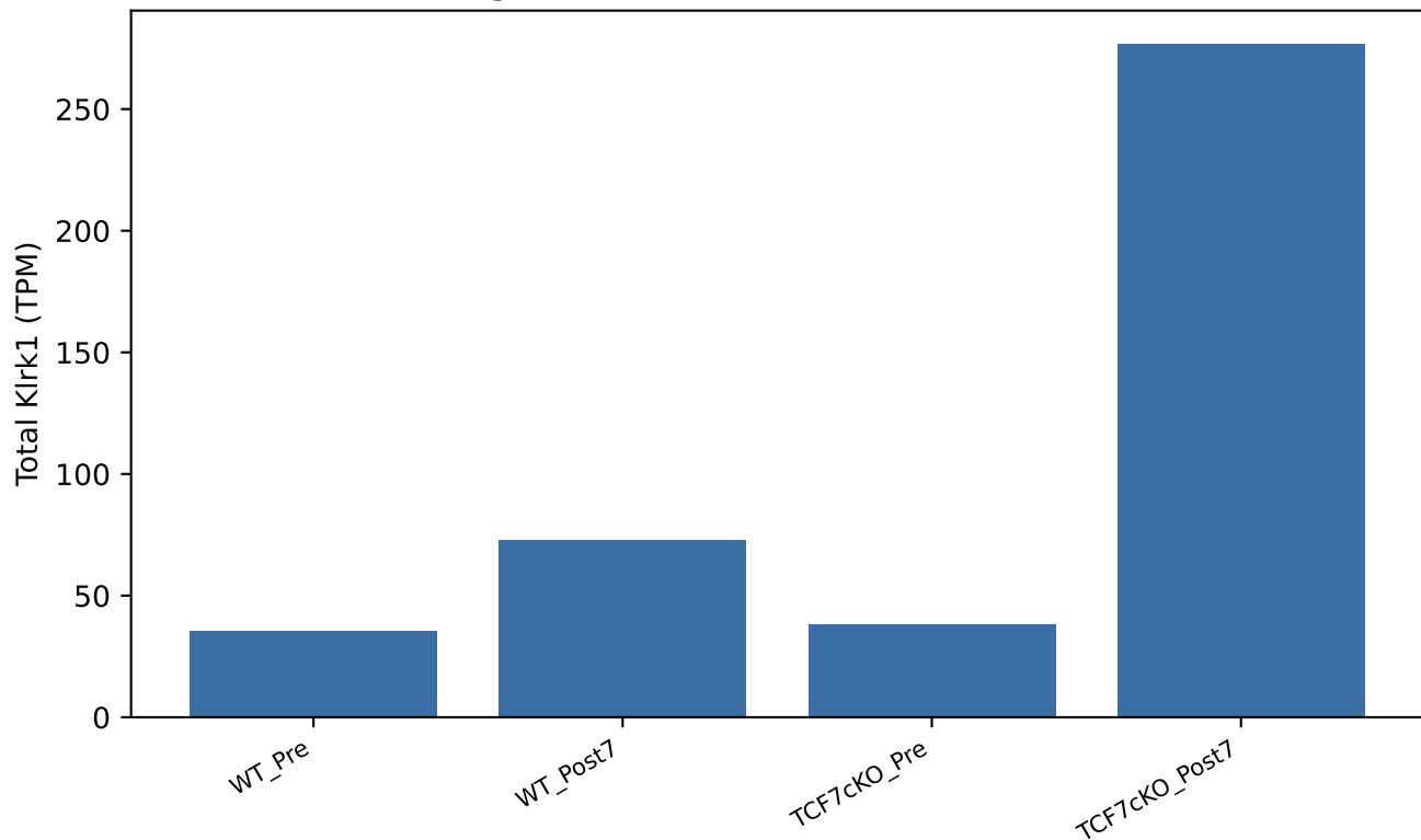
FigV2 — Total Klrk1 (GSE203167)
