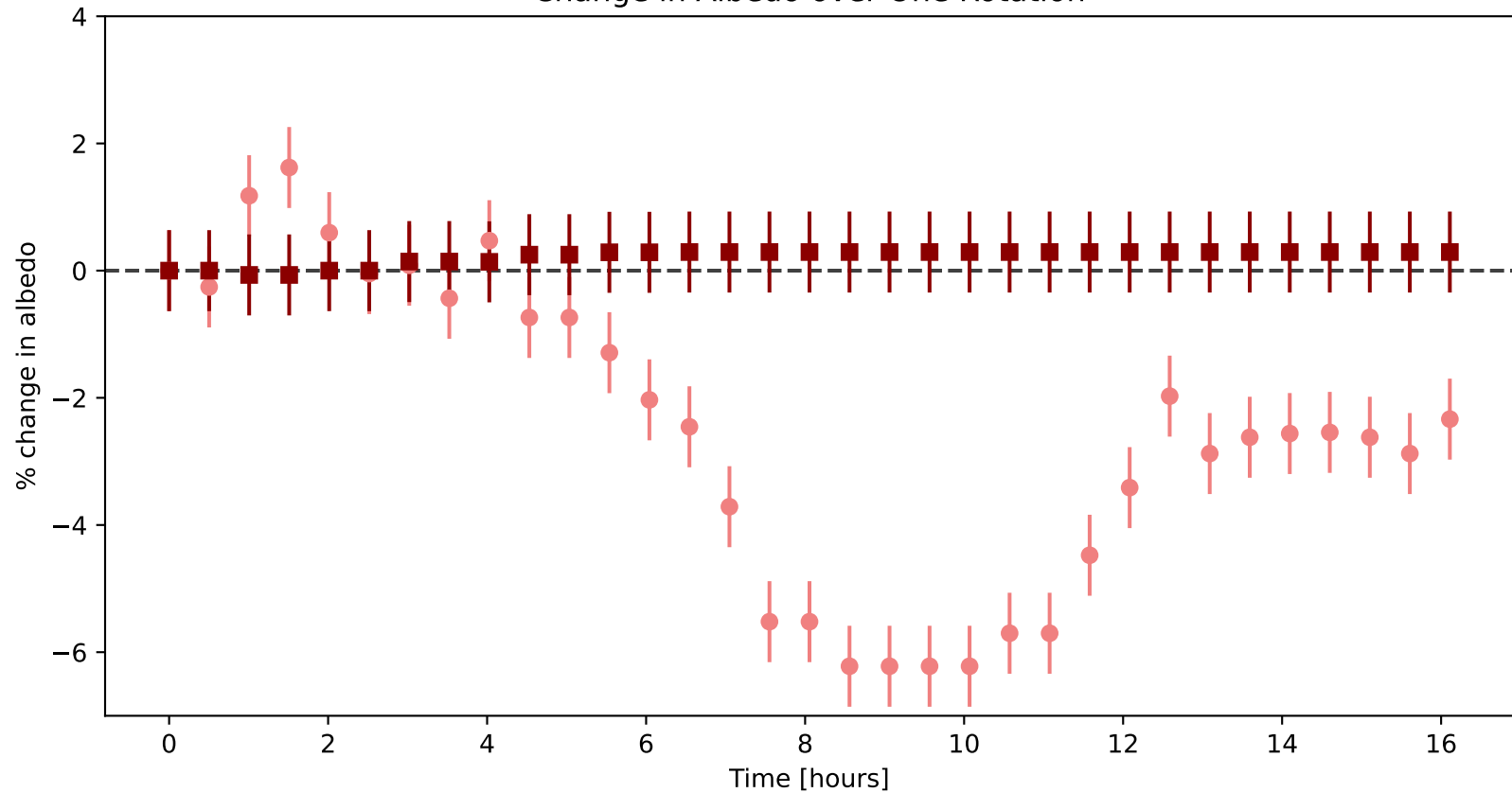
Change in Albedo over One Rotation
