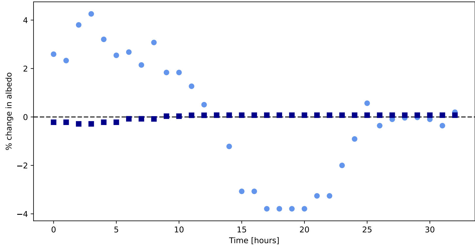
Change in Albedo over One Rotation
