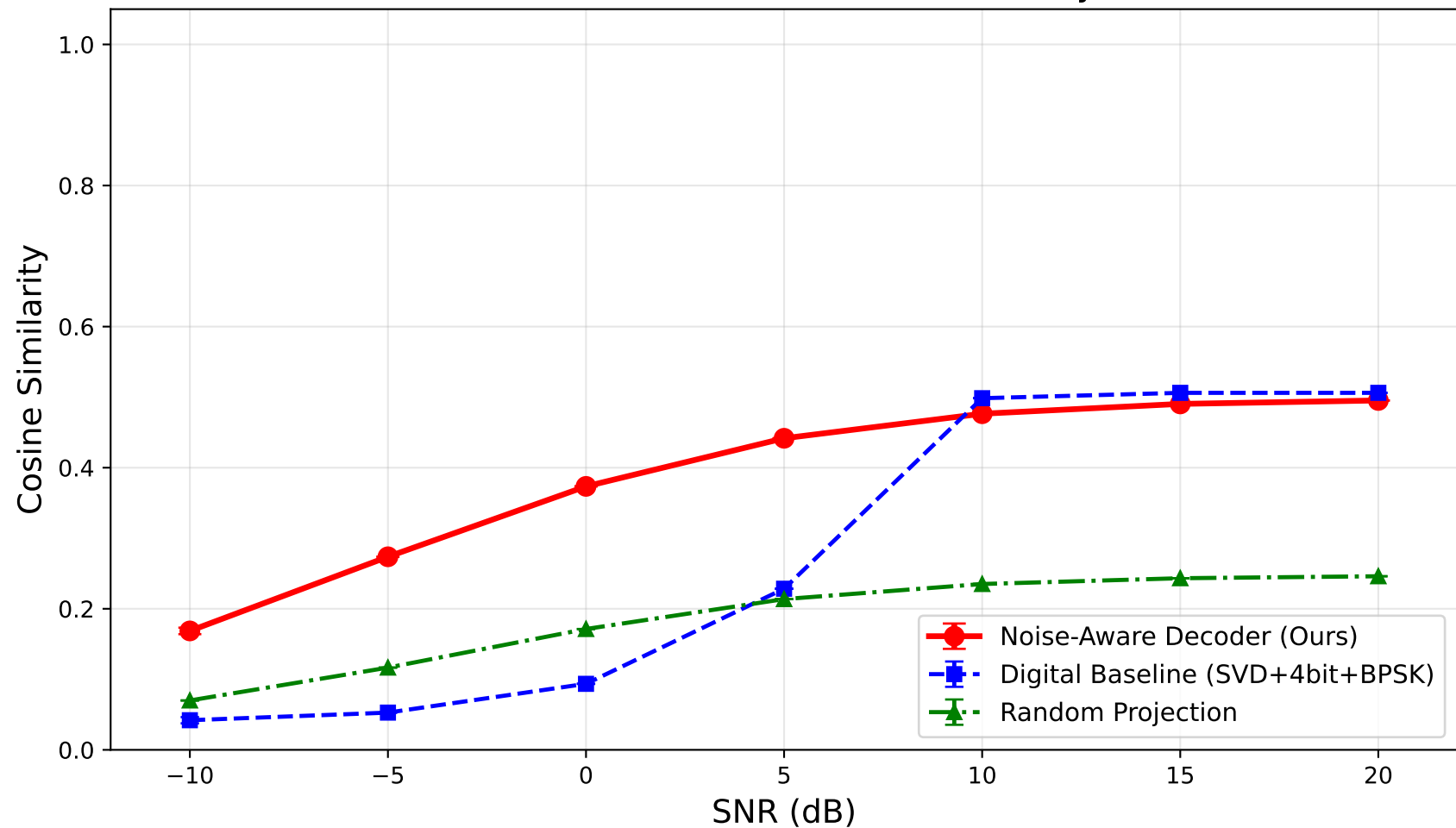
Semantic Communication: Cosine Similarity vs SNR
