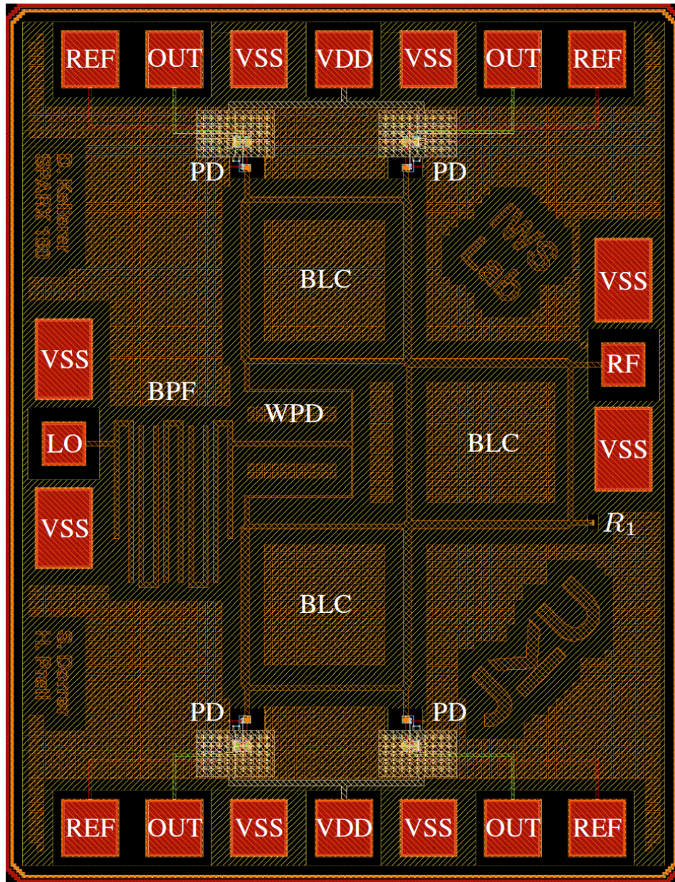
Figure 4: Chip render of the ihp-sgl3cmos six-port receiver for 160 GHz with M5 GND plane and pinout (1 mm \times 1.4 mm).
