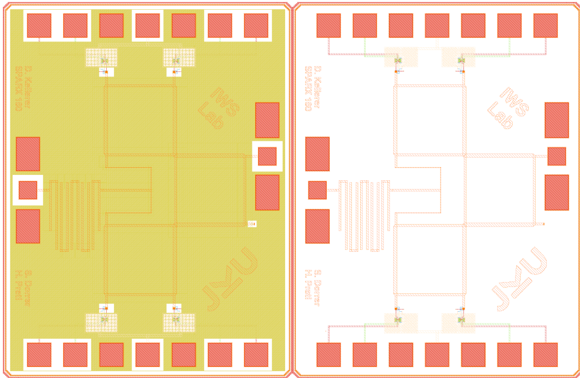
(a) 160 GHz layout with M5 GND plane
