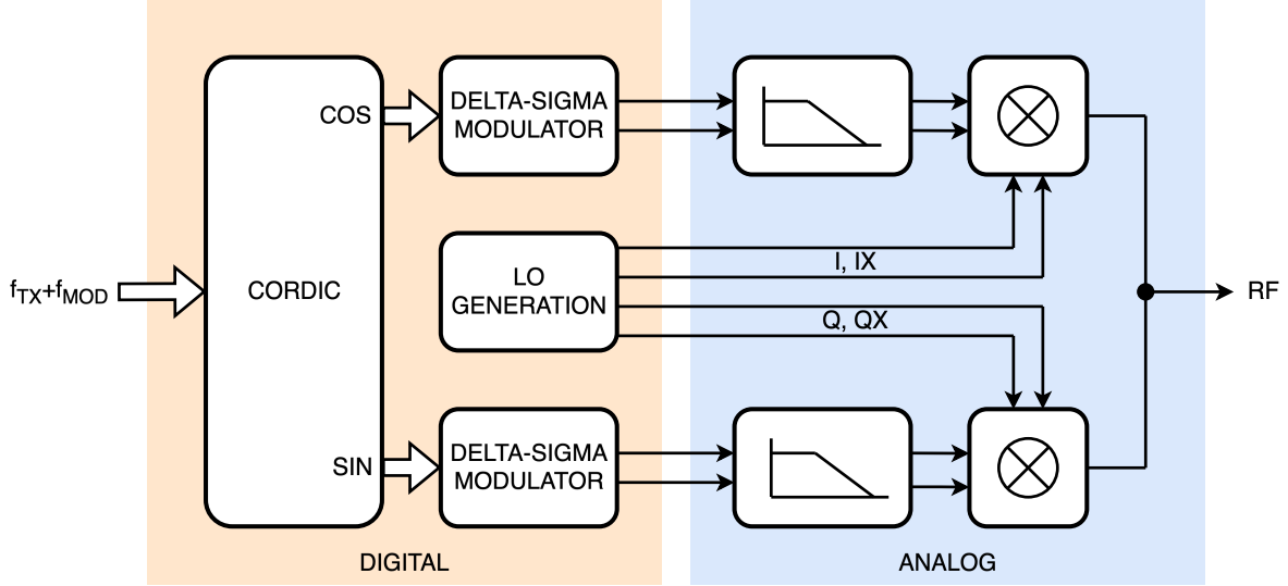
Figure 2: Architecture of the mixed-signal WSPR transmitter.
