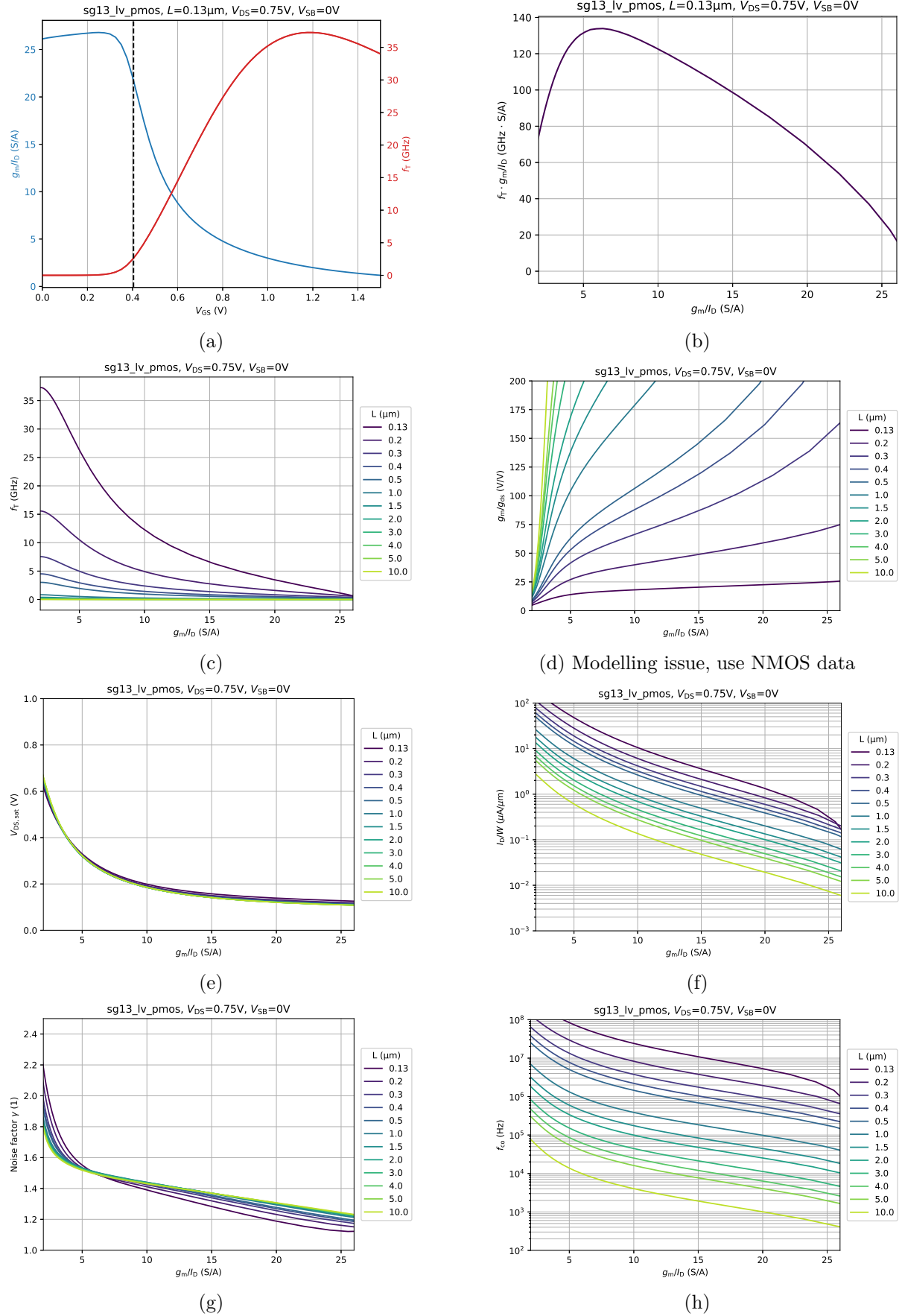
Figure 2: Characterization plots of SG13G2 LV PMOST for the g_m/I_D methodology.
