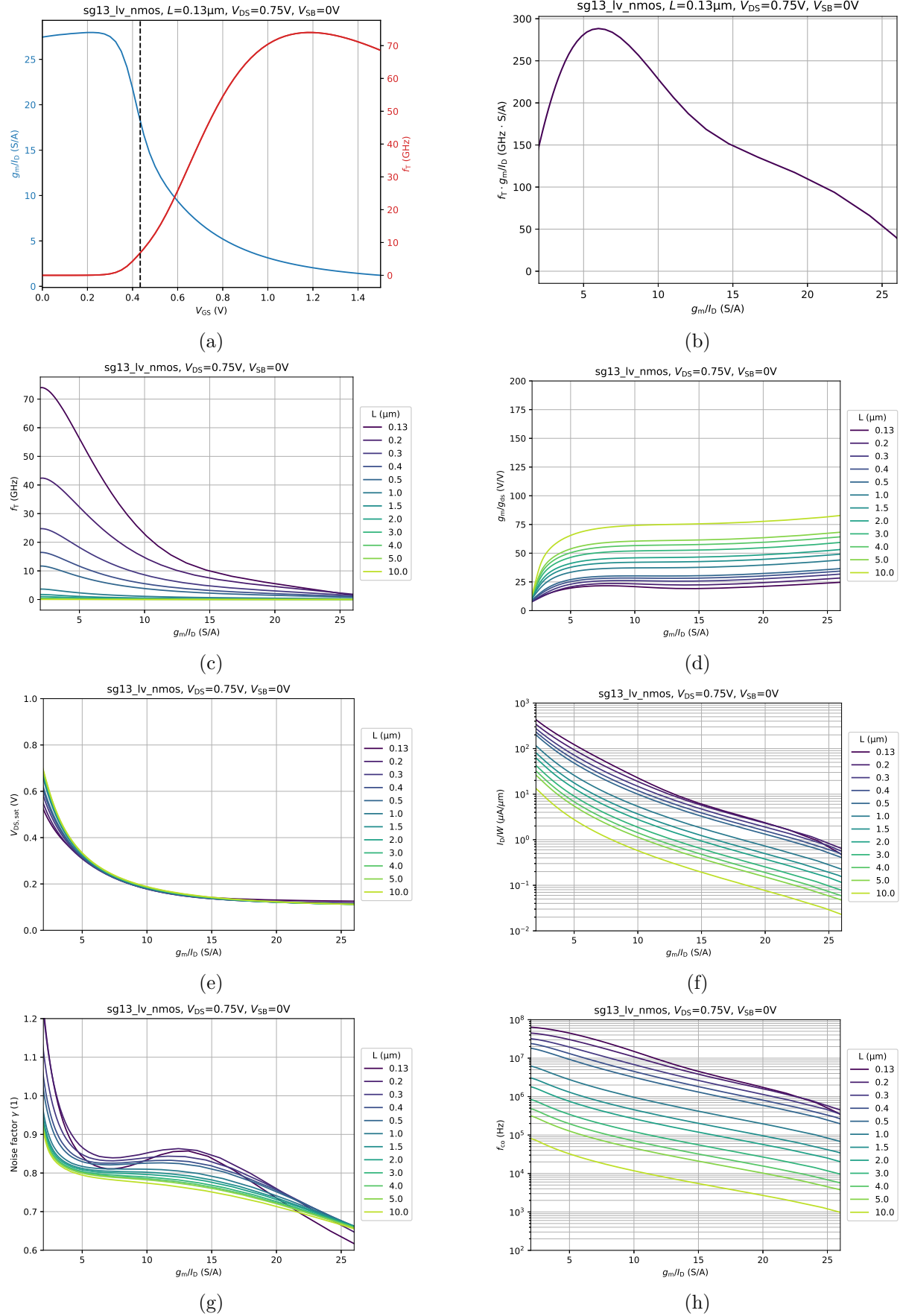
Figure 1: Characterization plots of SG13G2 LV NMOST for the g_m/I_D methodology.
