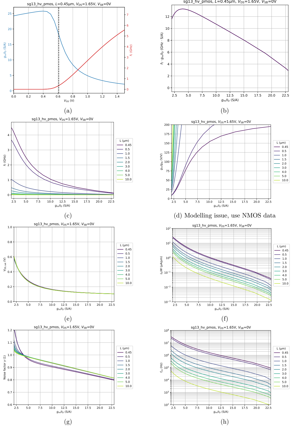
Figure 4: Characterization plots of SG13G2 HV PMOST for the g_m/I_D methodology.
