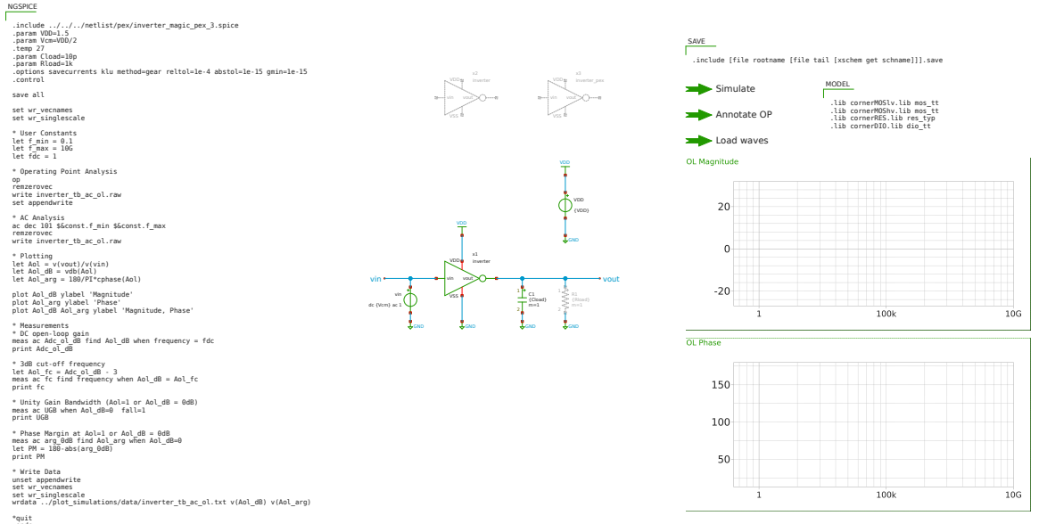
Figure 9: Xschem testbench inverter_tb_ac_ol (open-loop ac characterisation on inverter).
