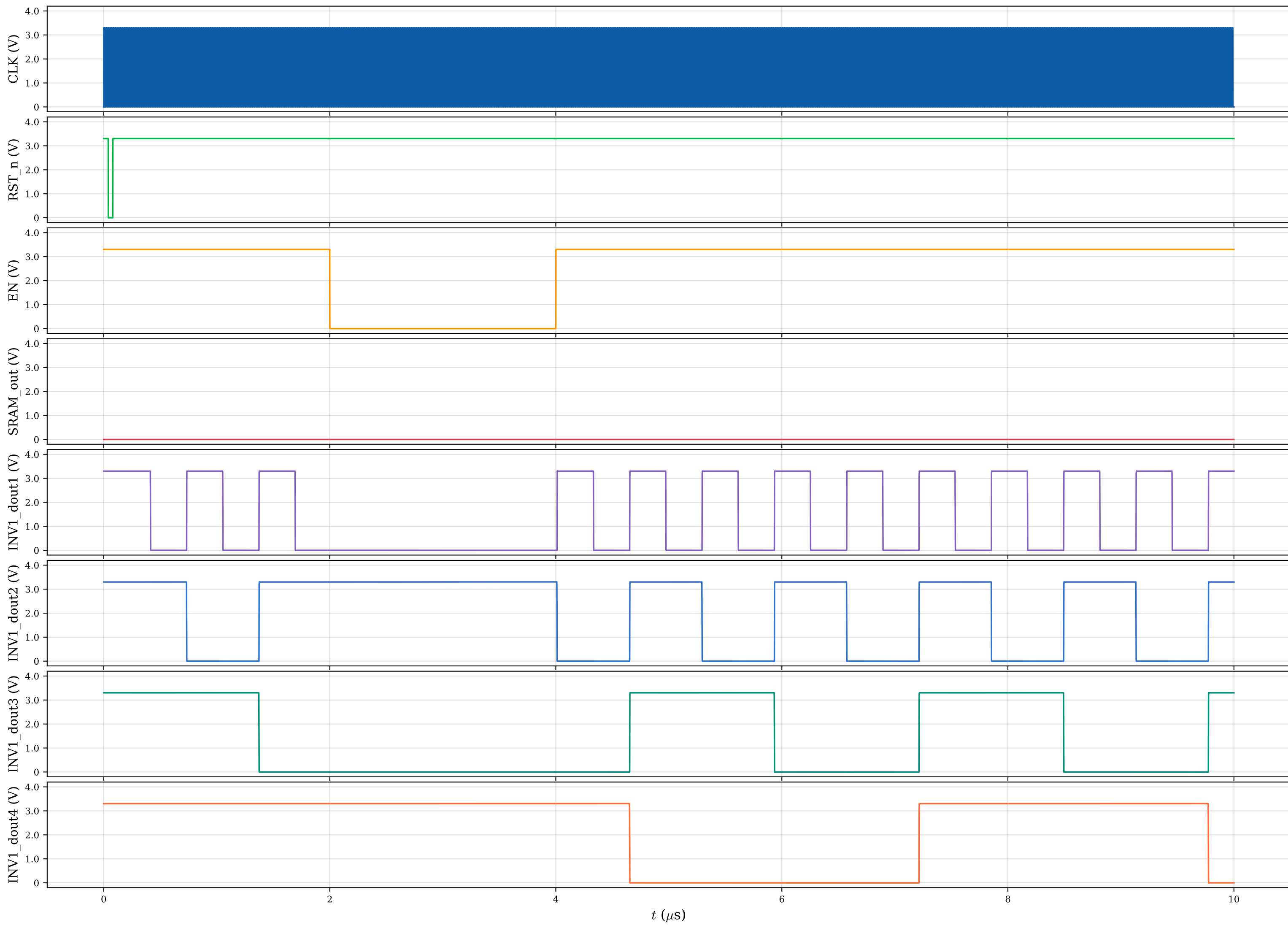
Chip Top — Digital Inverter Outputs (INV1)
