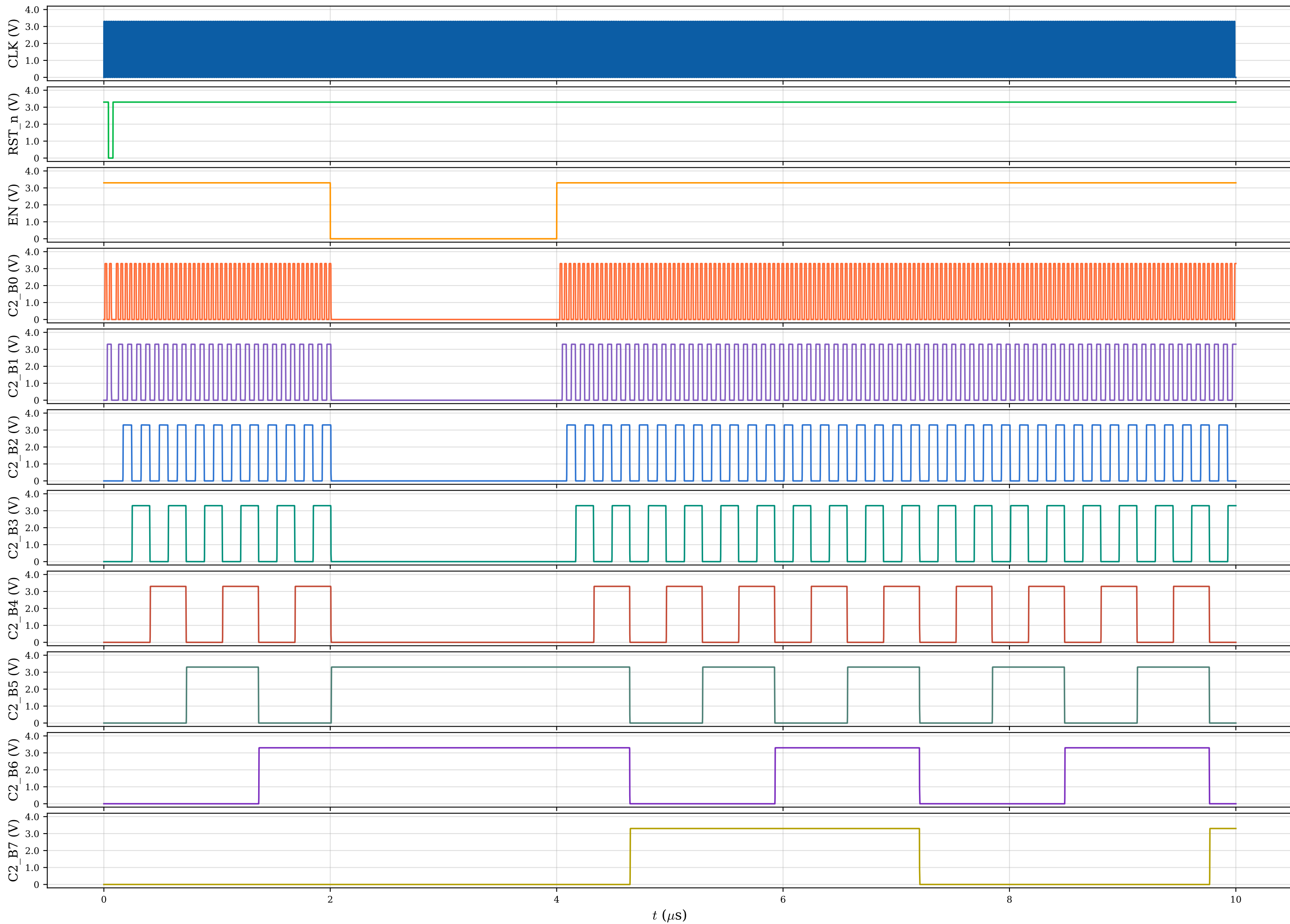
Chip Top — Counter 2 Output Bits
