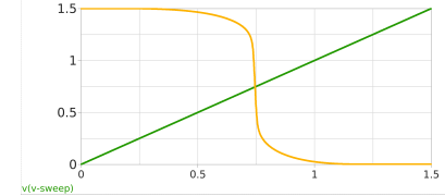
Figure 10: Xschem testbench inverter_tb_dc_vout (dc input sweep on inverter).
