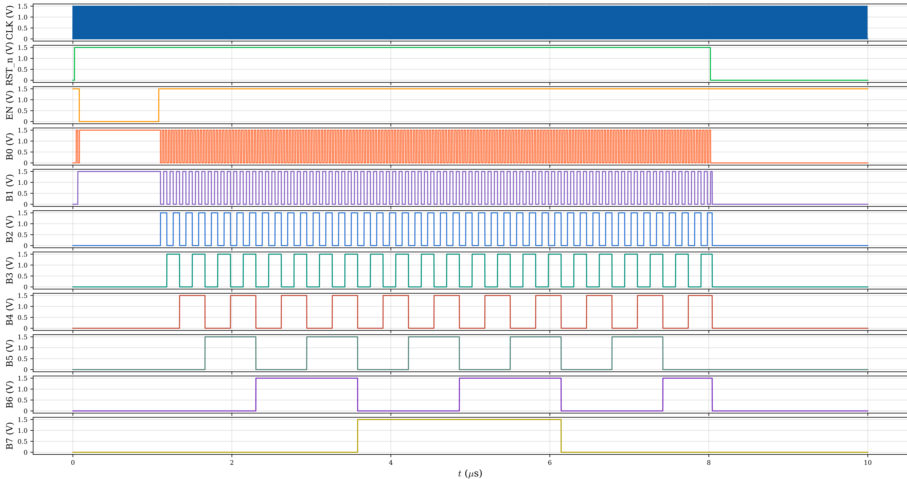
Counter Top - Gate-Level Transient Simulation
