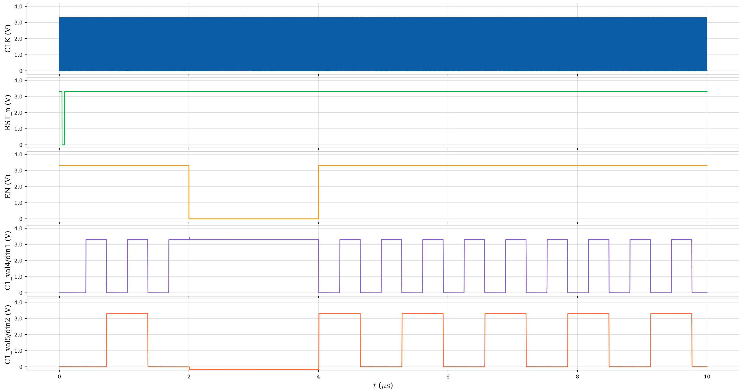
Chip Top — Counter 1 / INV1 Inputs (Bits 4-5)
