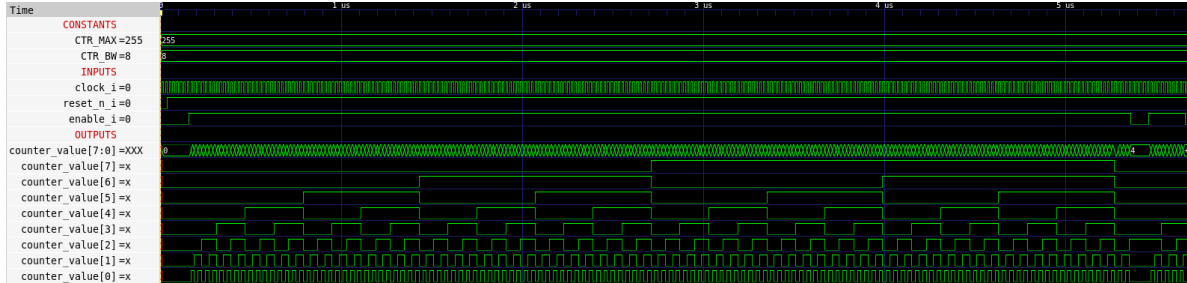
Figure 3: RTL Verilog waveform of counter_top in GTKWave.
