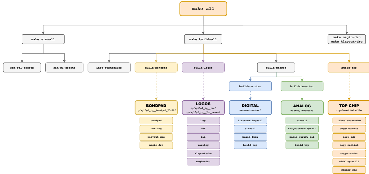
Figure 2: Overview of the Makefile targets that make all resolves to. Every coloured branch corresponds to one deliverable (top chip, bondpad, logos, digital macro, analog macro). The grey targets connect make all to those branches.
