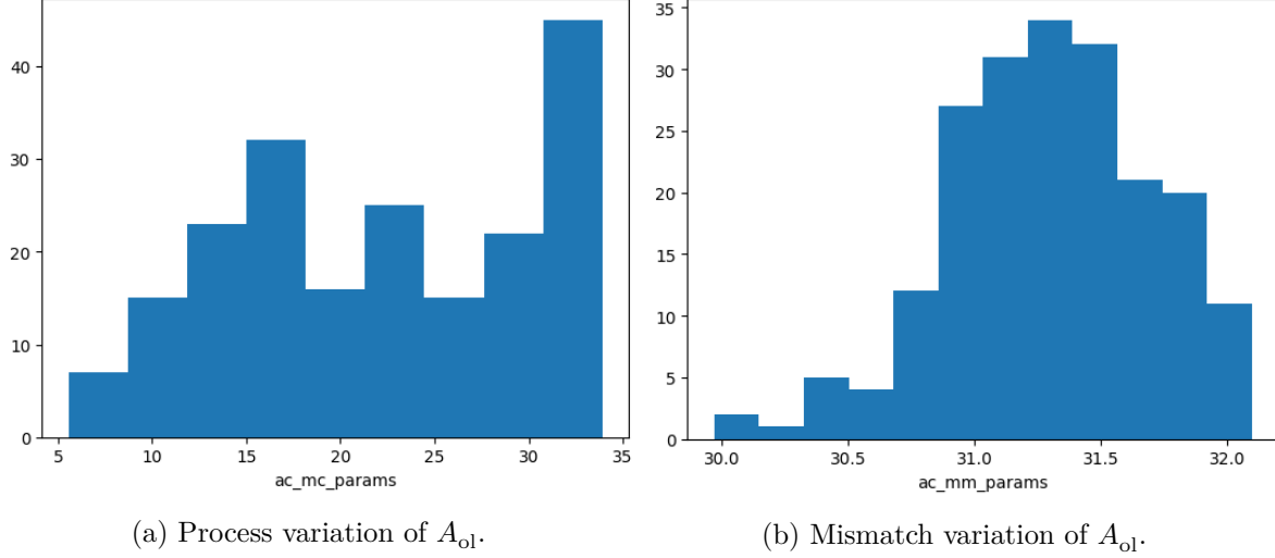
Figure 17: CACE process (left) and mismatch (right) variations of A_{ol} .
