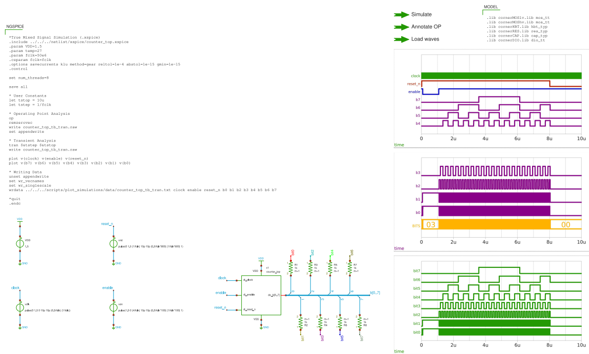
Figure 6: Xschem mixed-signal gate-level testbench counter_top_tb_tran .
