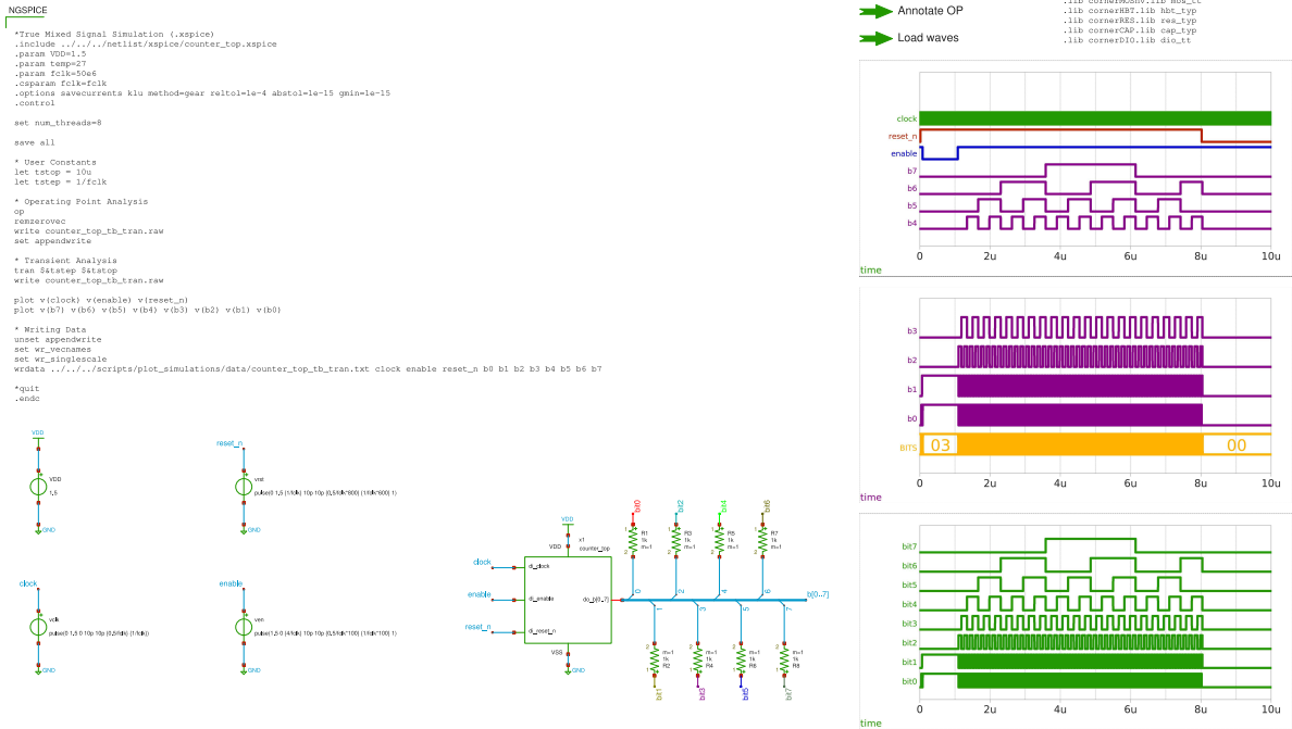
Figure 6: Xschem mixed-signal gate-level testbench counter_top_tb_tran.
