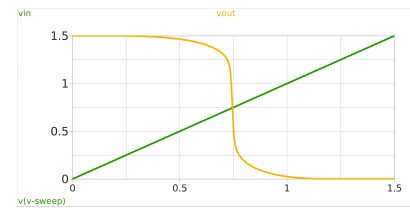
Figure 10: Xschem testbench inverter_tb_dc_vout (dc input sweep on inverter).
