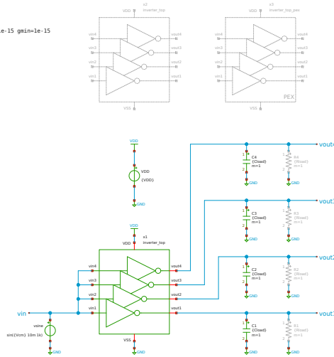
Figure 11: Xschem top-level testbench inverter_top_tb_tran (transient on inverter_top).
