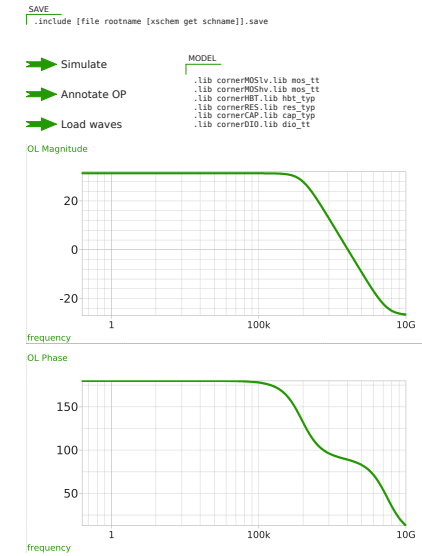
Figure 9: Xschem testbench inverter_tb_ac_ol (open-loop ac characterisation on inverter).
