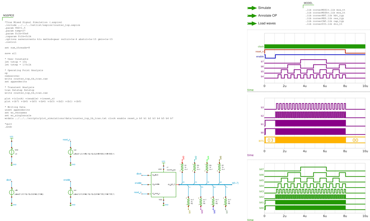
Figure 6: Xschem mixed-signal gate-level testbench counter_top_tb_tran.
