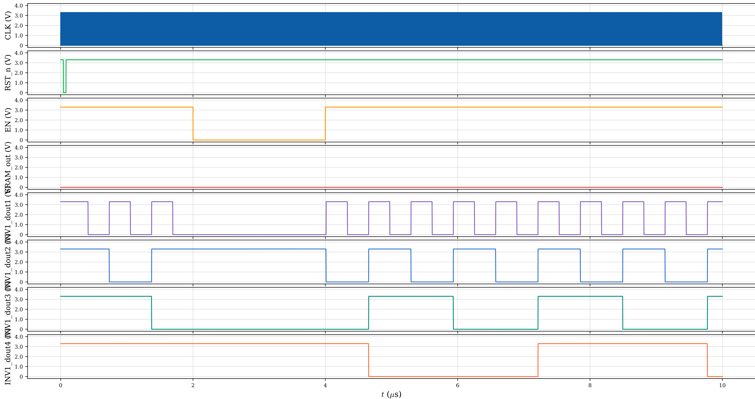
Chip Top — Digital Inverter Outputs (INV1)
