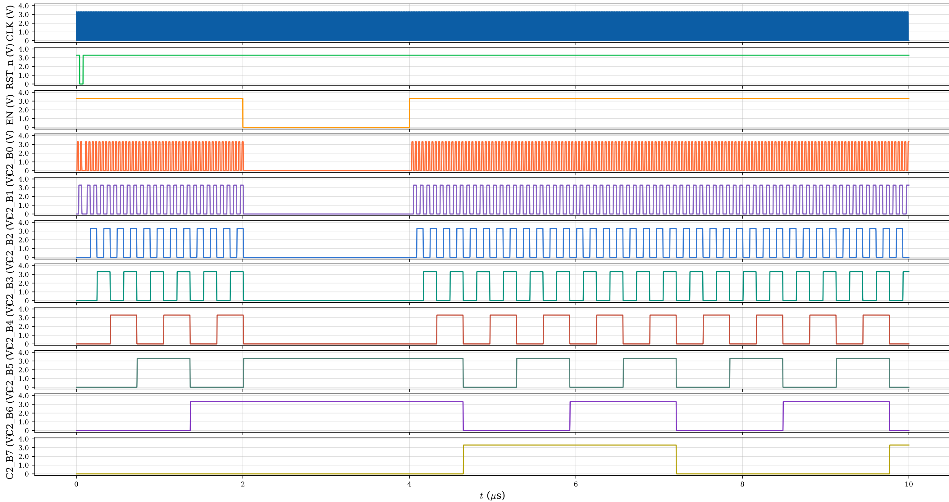
Chip Top — Counter 2 Output Bits
