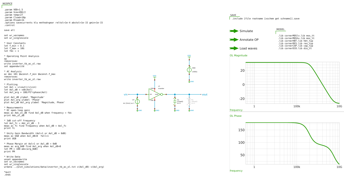
Figure 9: Xschem testbench inverter_tb_ac_ol (open-loop ac characterisation on inverter).
