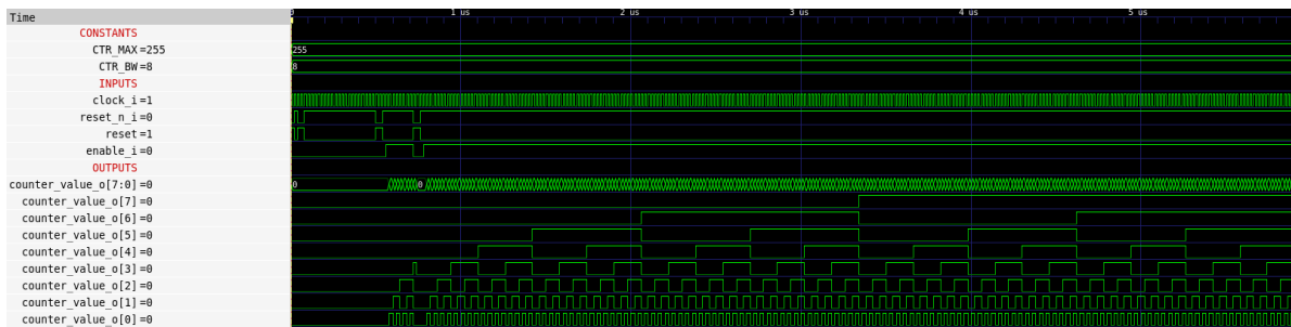
Figure 4: Gate-level cocotb waveform of counter_top in GTKWave.
