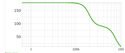
Figure 9: Xschem testbench inverter_tb_ac_ol (open-loop ac characterisation on inverter).
