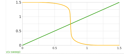
Figure 10: Xschem testbench inverter_tb_dc_vout (dc input sweep on inverter).
