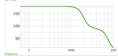
Figure 9: Xschem testbench inverter_tb_ac_ol (open-loop ac characterisation on inverter).
