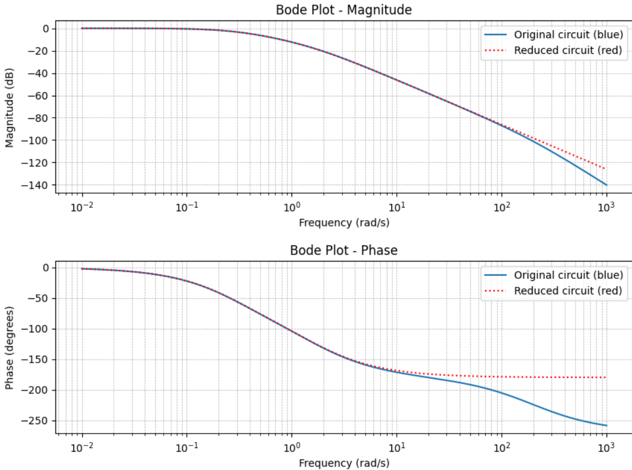
Figure 34: Bode Plots
