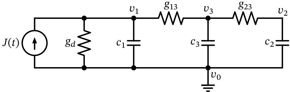
Figure 39: Passive RC circuit shown in Sheehan (2007).
