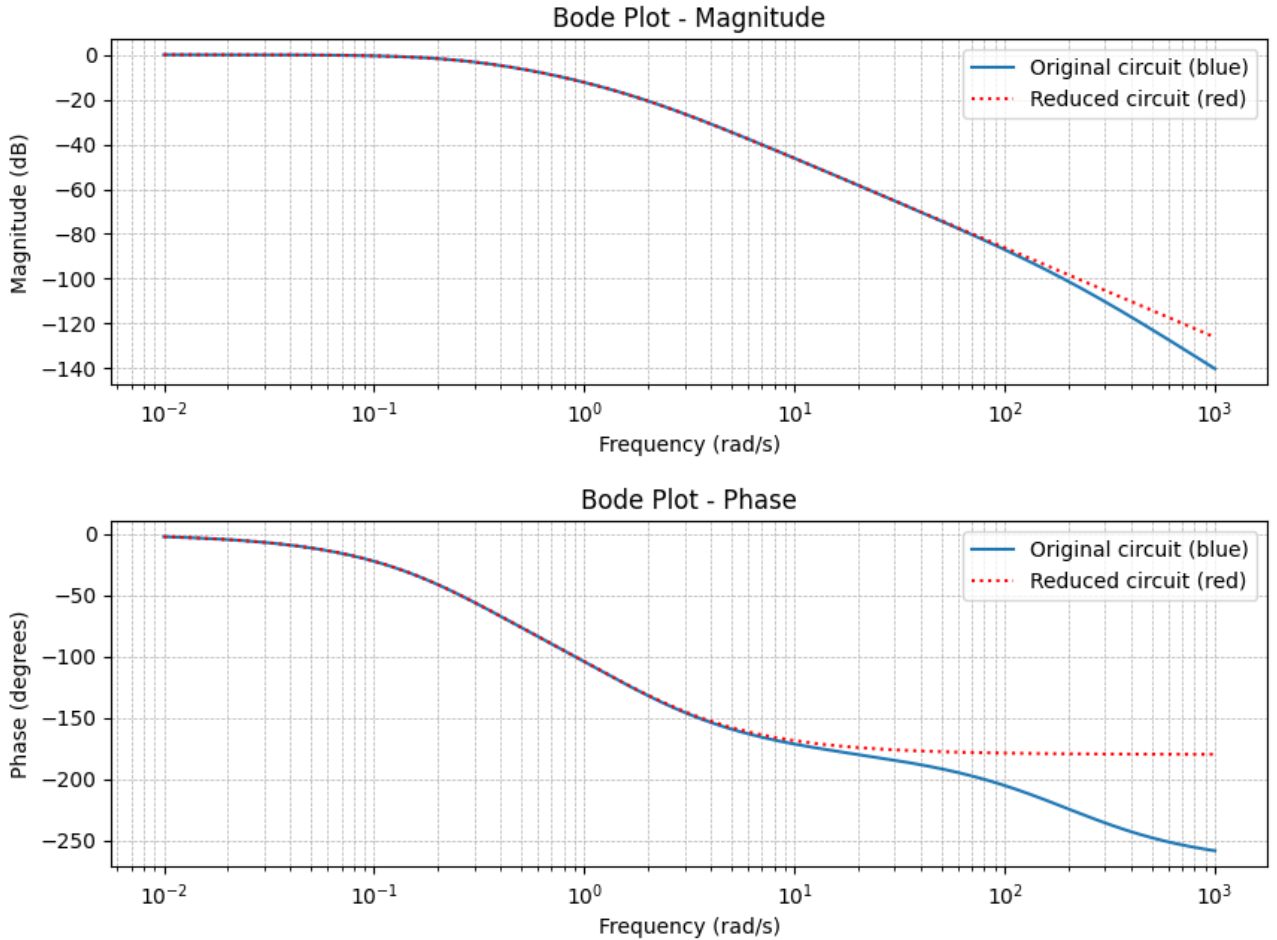
Figure 41: Bode Plots
