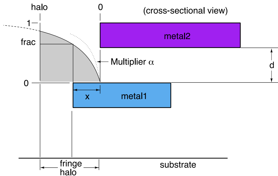
Figure 15: Fringe Capacitance: Overlapping (2)
