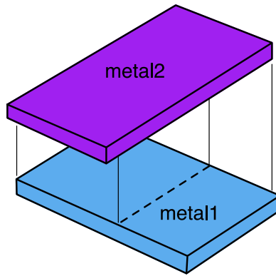
Figure 13: Overlap Capacitance
