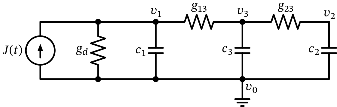
Figure 39: Passive RC circuit shown in Sheehan (2007).
