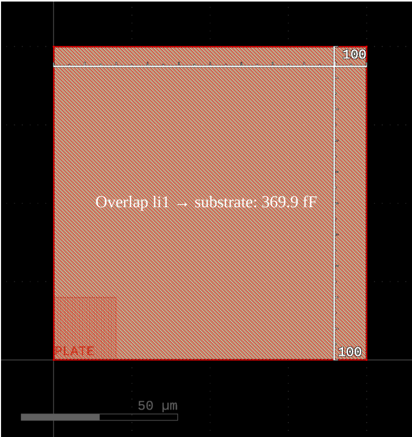
Figure 22: Overlap capacitance li1 to substrate.
