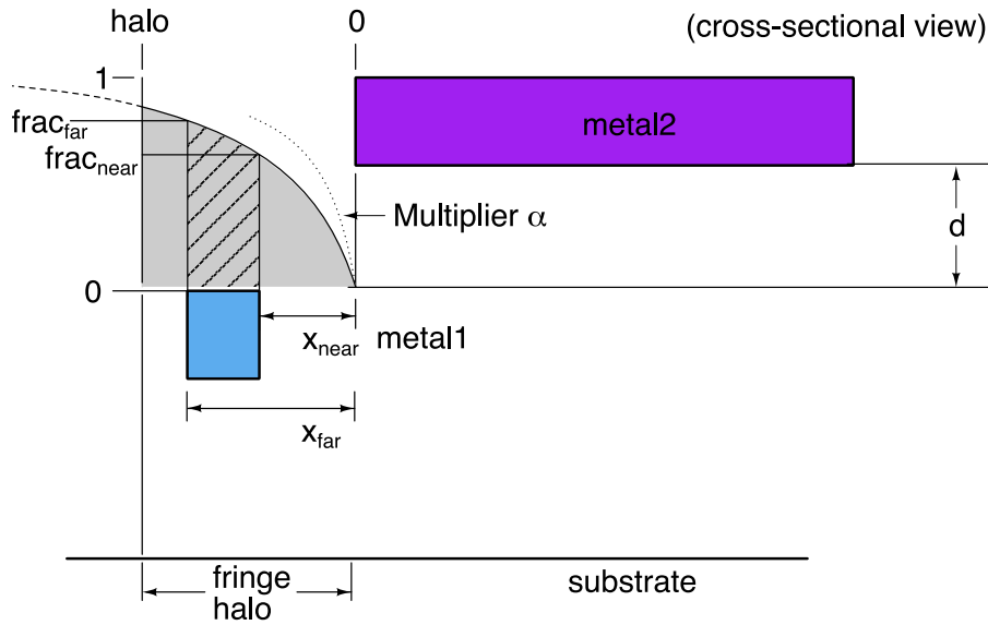
Figure 17: Fringe Capacitance: Non Overlapping (2)
