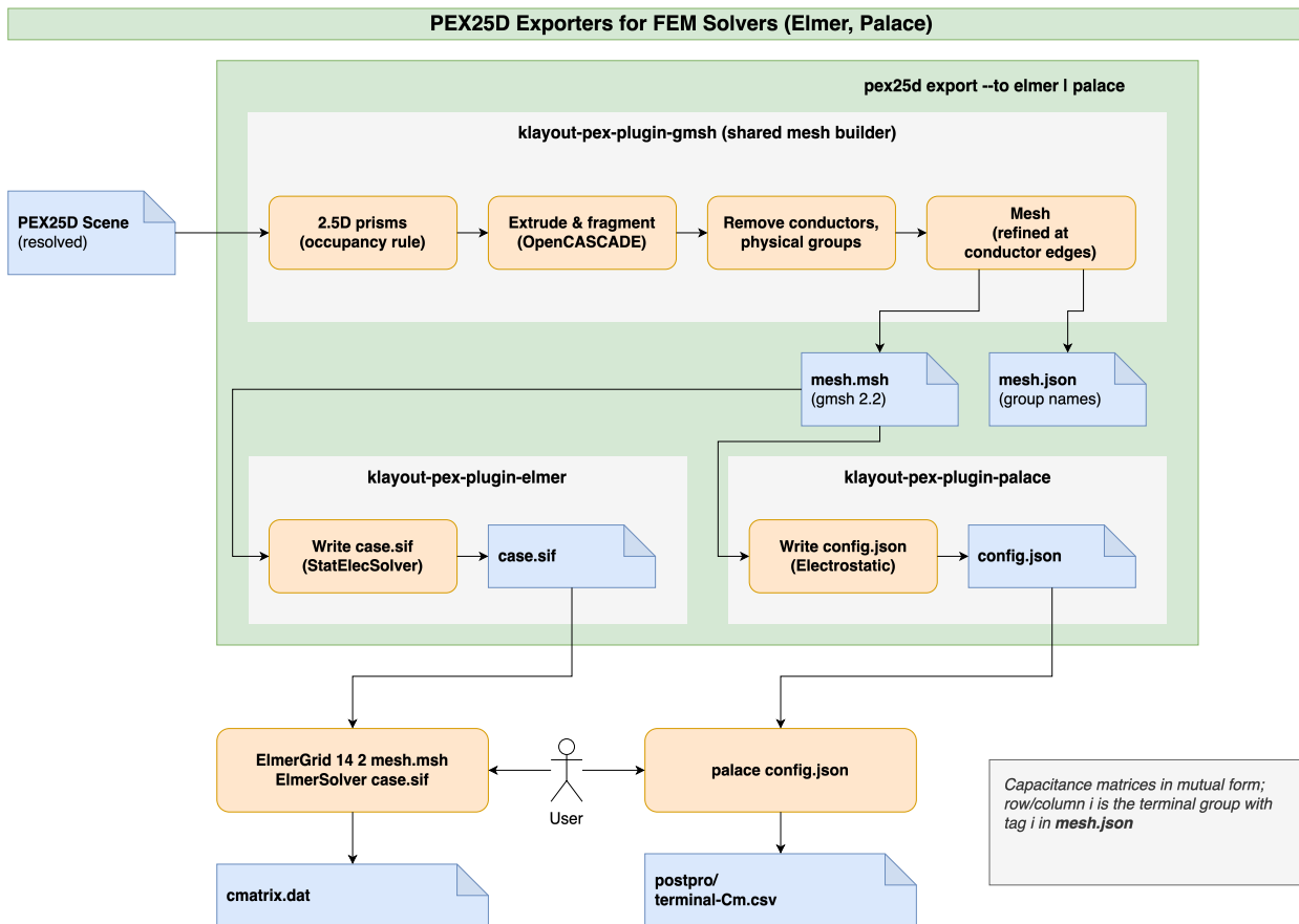
Figure 44: PEX25D Exporters for FEM Solvers
