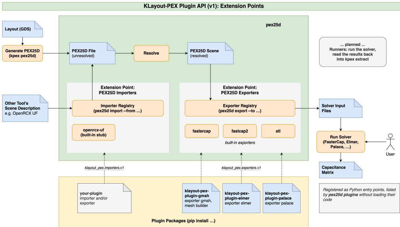
Figure 43: KPEX Plugin API: Extension Points
